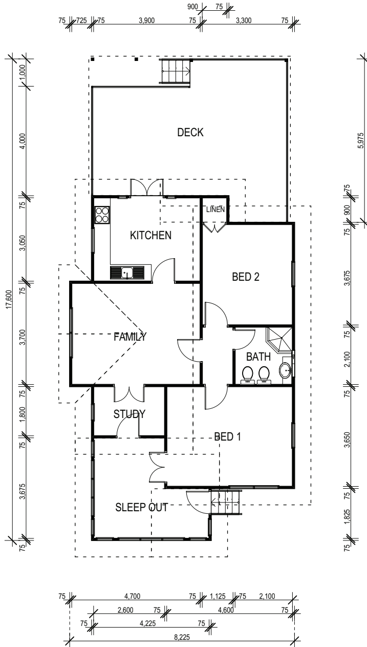
1 EXIST/DEMO FLOOR PLAN - FLOOR LEVEL L01 SCALE @ A3 1:100
