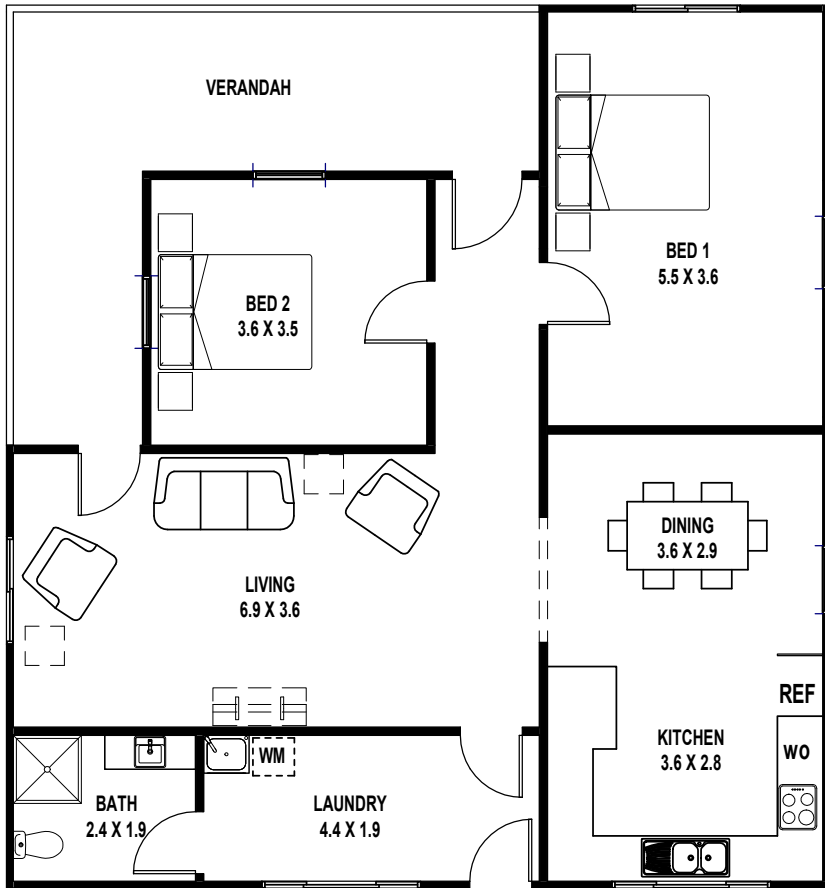
1 Floor Plan (Existing) Scale: 1 : 100
