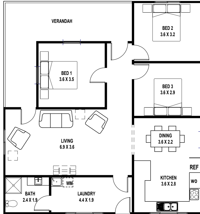
2 Floor Plan (Proposed) Scale: 1 : 100
